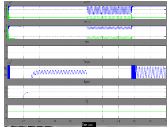
Fig 10. Output voltage, torque, speed at With statcom 1ph-60 % -Coordinated Positive -Negative Sequence Compensation
