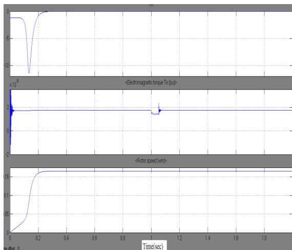
Fig 6. Simulink output of the wind farm at Without StatCom- 1ph-50 % with
