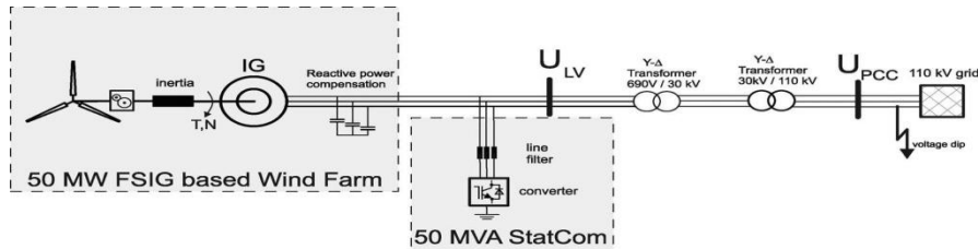
Fig. 1. Structure of the investigated system: FSIG-based wind farm and StatCom connected to the grid
