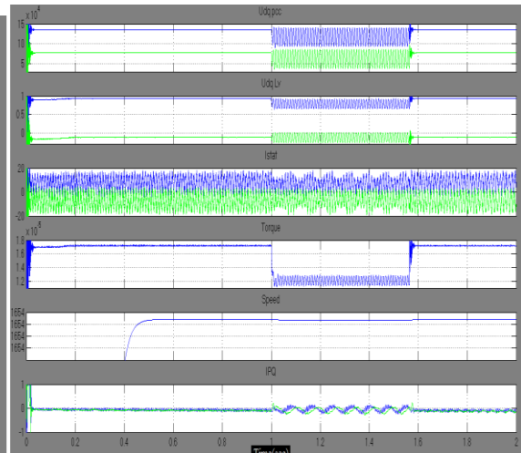
Fig 7. No load voltage, output voltage, StatCom current, torque, speed, active and reactive power at StatCom –1ph-50 % -Positive Sequence Compensation
