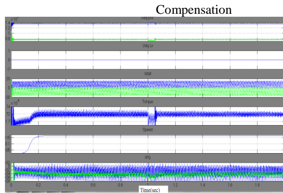
Fig 11. StatCom -1ph-0 % -Coordinated Positive -Negative Sequence Compensation
