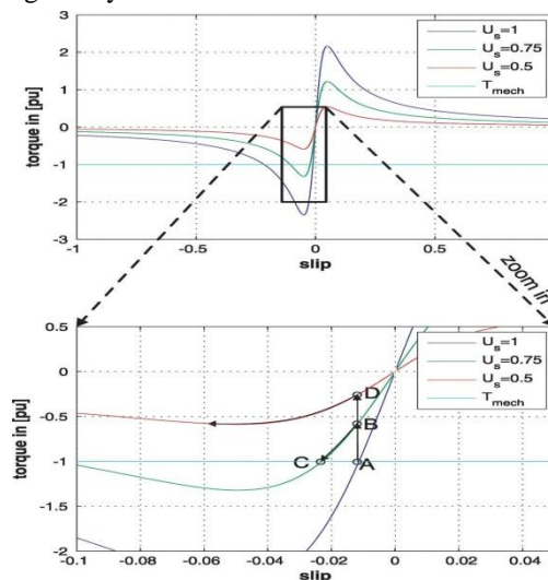
Fig. 2. Theoretical torque-slip characteristics of the induction generator under different grid voltage levels
