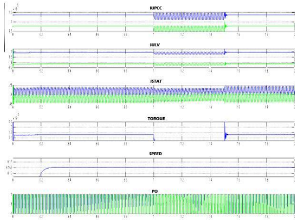
Fig 9. Output at With StatCom -1ph-50 % -Negative Sequence Compensation Sequence
