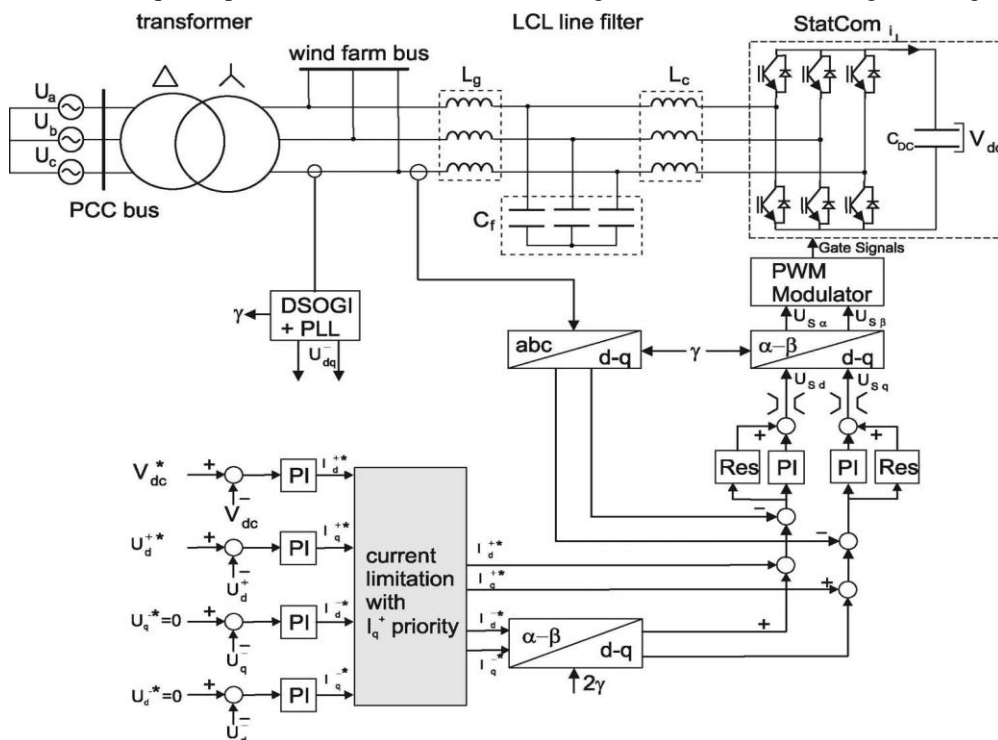
Fig. 3. Proposed control structure of the StatCom to control the positive- and the negative-sequence voltage independently
