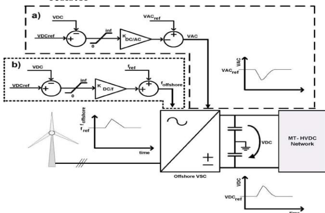
Fig. 4. Control scheme for FRT provision based on dc voltage: (a) AC offshore grid voltage control. (b) AC offshore grid frequency control.
