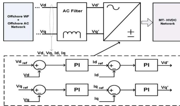
Fig. 1. Internal control loops of the offshore converters
