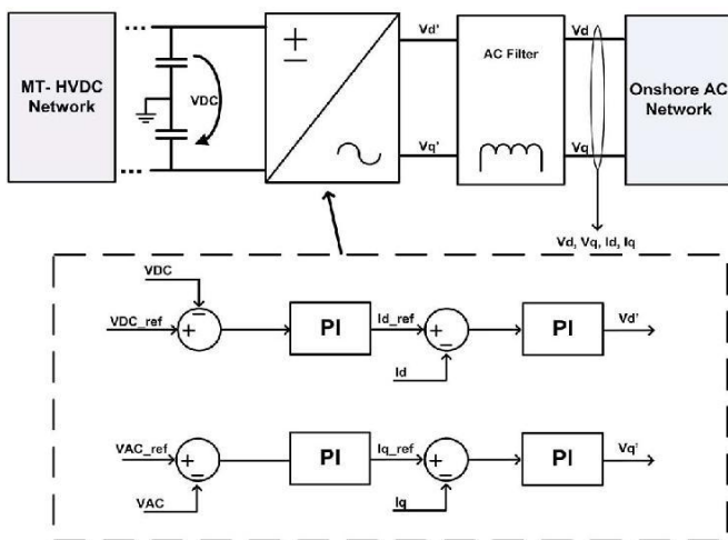
Fig. 2. Internal control loops of the onshore converters
