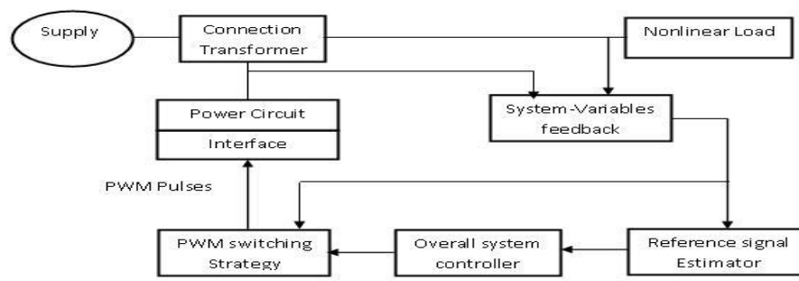
Fig 2. Block diagram of active power filter operation
