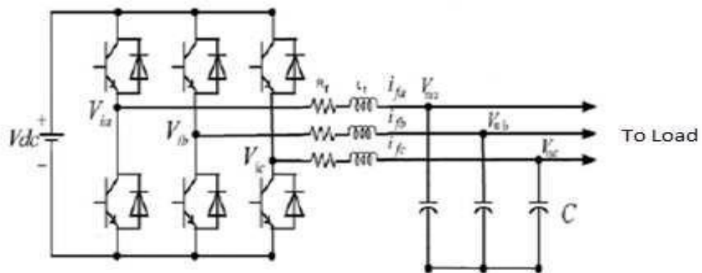
Fig 1. PWM interfacing inverter
