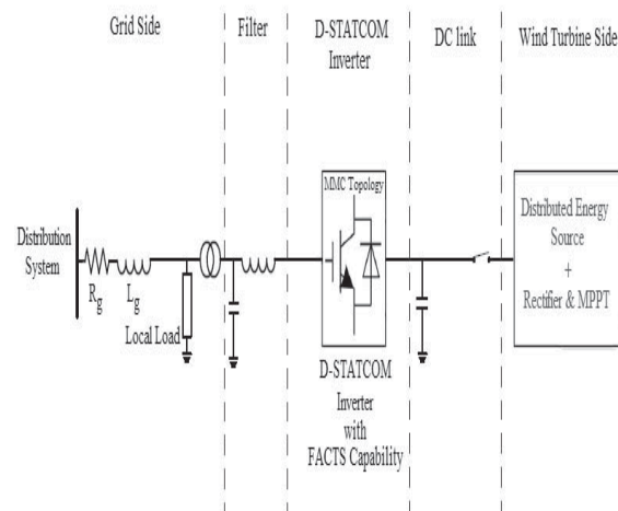
Fig. 1. Complete configuration of the proposed inverter with FACTS capability
