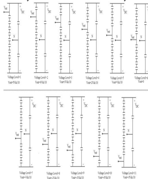
Fig. 5. Selection of SMs' capacitors for different voltage levels.
