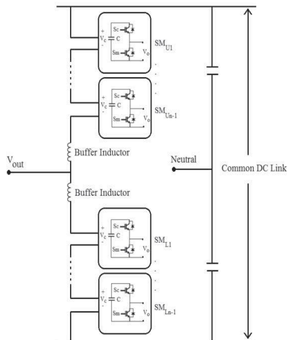
Fig.2. Structure of a single-phase MMC inverter structure
