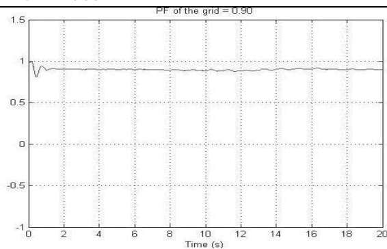
Fig. 9. Simulated PF of the grid.
