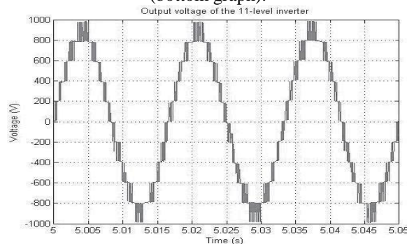
Fig. 8. Simulated output voltage of an 11-level inverter.
