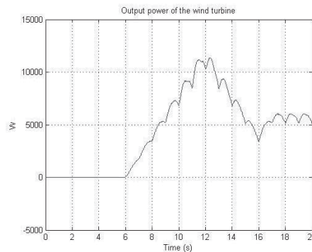
Fig. 6. Simulated output active power from the wind turbine.
