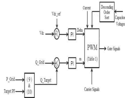
Fig. 3 Schematic of the proposed controller system
