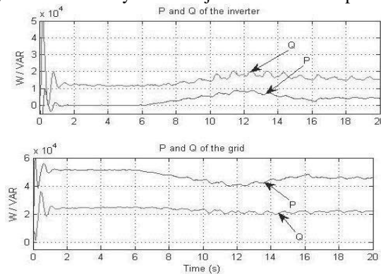
Fig. 7. Simulated active and reactive power of the inverter (top graph), active and reactive power of the power lines (bottom graph).
