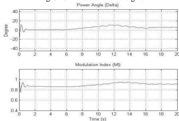
Fig. 10. Simulated delta and modulation index of the 11-level inverter.
