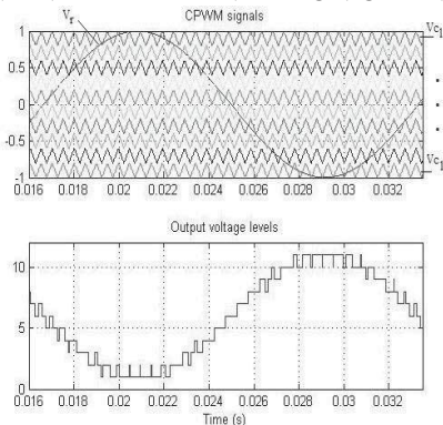
Fig. 4. CPWM waveforms for an 11-level MMC inverter, and the generated output voltage level
