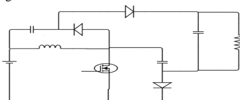
Fig.4 Inductor and exchanged capacitor topologies (IEC)
