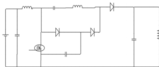
Fig.3 Topologies with Coupled inductor (CI)
