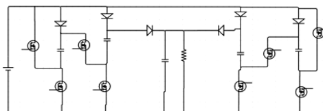
Fig.2 Topologies with Switched capacitor (SC)
