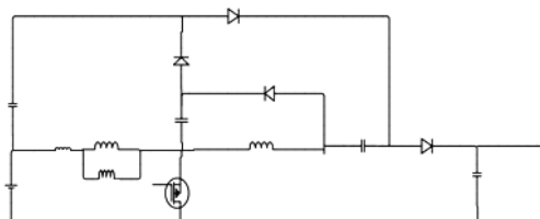
Fig.5 Coupled inductor and exchanged capacitor topologies (CIEC)
