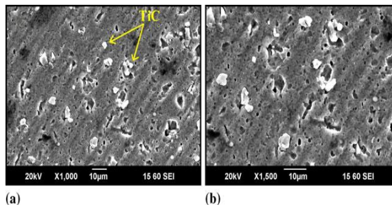
Fig 12. (a) and (b) SEM photomicrograph of AA1050/TiC SMMC.
