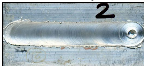
Figure 9. Crown appearance of FSP zone of AA1050/TiC SMMC.
