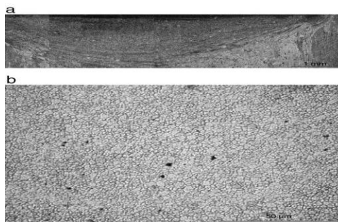
Fig. 4. Macrograph of the stirred zone (a) and Nugget zone equiaxed recrystallized grains after the dynamic recrystallization process (b).
