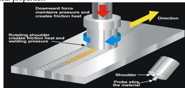
Fig 1. Schematic illustration of friction stir processing
