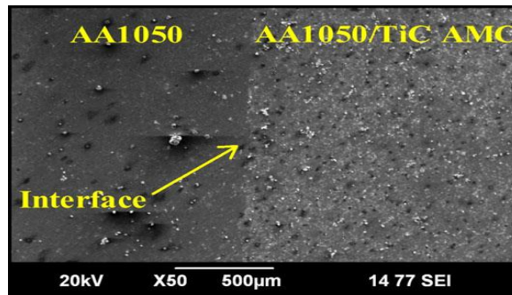
Fig 11. SEM photomicrograph of interface zone.
