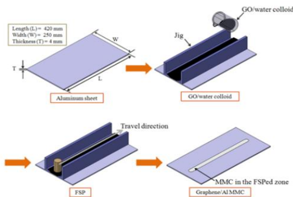
Fig. 14 a schematic of MMC fabrication by FSP
