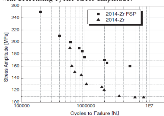
Fig. 5. Fatigue endurance S–N curve of the studied material in FSP and as-extruded conditions.
