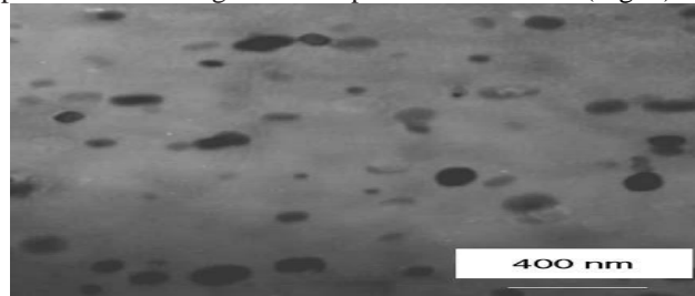
Fig. 3. Al_3Zr precipitates observed in the studied material
