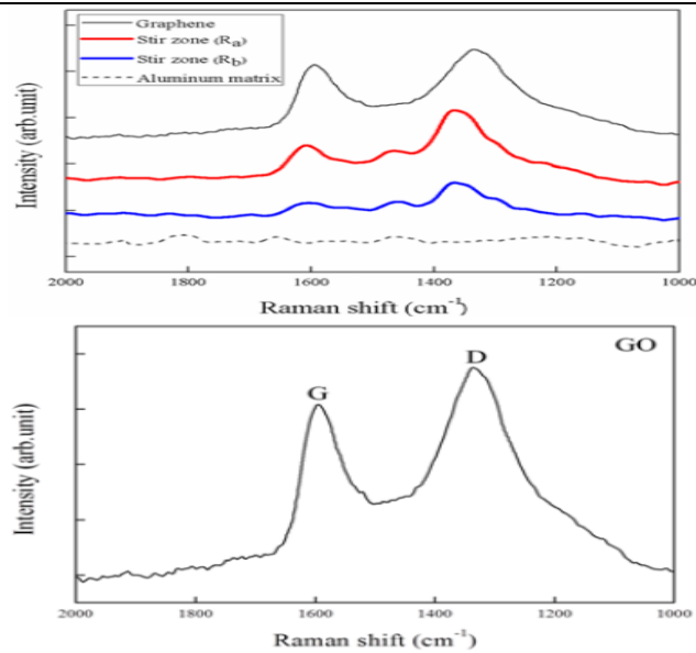
Fig. 16a. Raman spectrum of GO and 16.b Raman spectrum of Graphene /Al MMC
