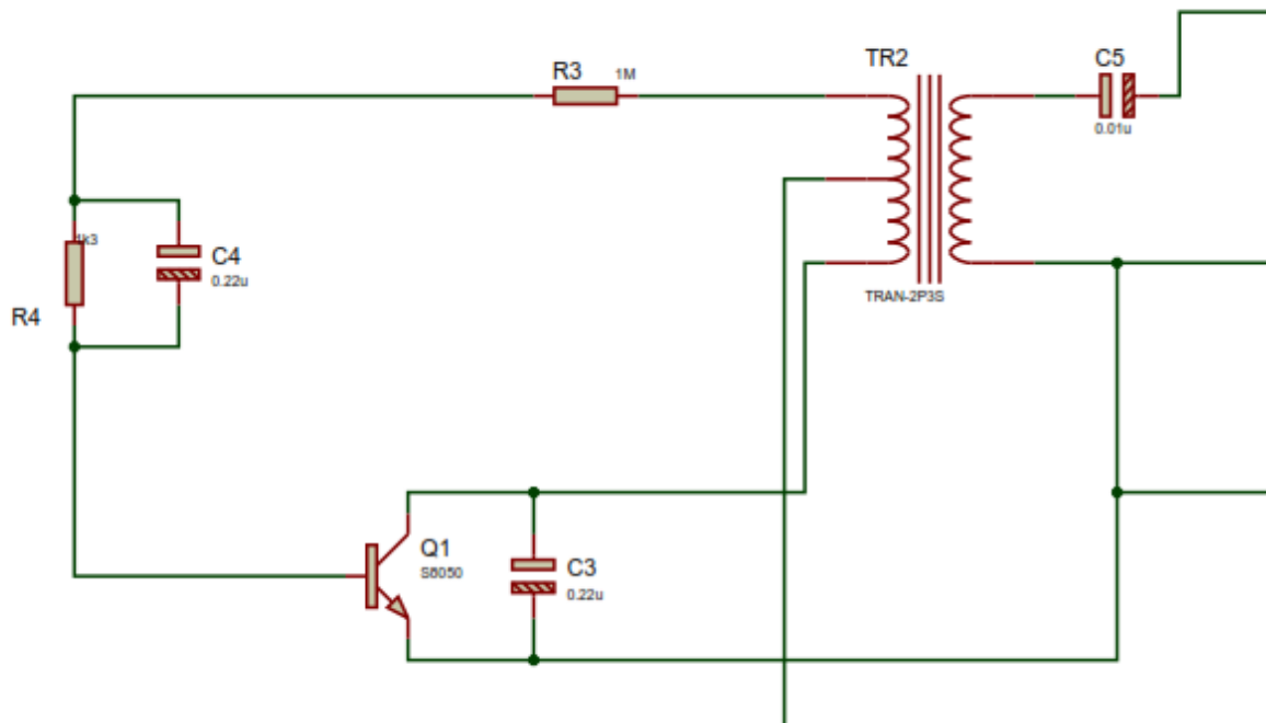
Figure 1.4 One Transistor Inverter amplifiers
