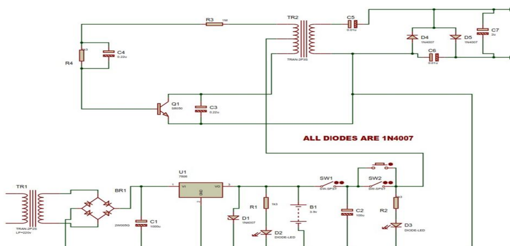
Fig. 1.1 General Zapper circuit diagram
