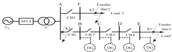
Fig. 2. Application of the active SFCL in a distribution system with DG units.
