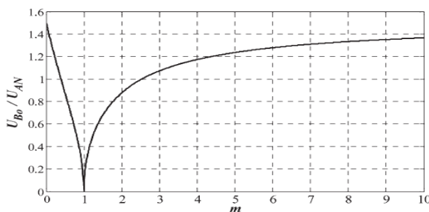
Fig. 3. Relationship between the reactance ratio m and the B-phase overvoltage.
