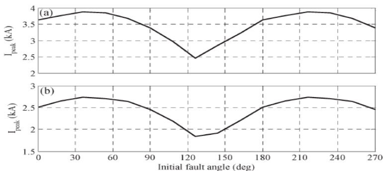
Fig. 7. Influence of initial fault angle on the peak amplitude of the A-phase short-circuit current. (a) Without SFCL and (b) with the active SFCL.
