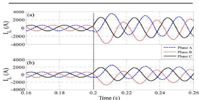
Fig. 5. Line current waveforms when the three-phase short-circuit occurs at k_3 point. (a) Without SFCL and (b) with the active SFCL.
