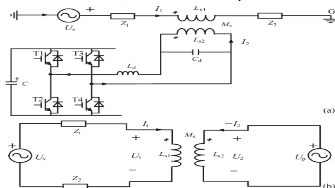
Fig. 1. Single-phase voltage compensation type active SFCL. (a) Circuit structure and (b) equivalent circuit.
