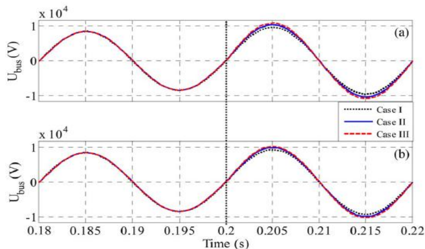
Fig. 4. Voltage characteristics of the Bus-A under different locations of DG units. (a) Without SFCL and (b) with the active SFCL.
