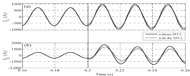
Fig. 6. Active SFCL's current-limiting performances under different fault locations. (a) k 1 point and (b) k 2 point.
