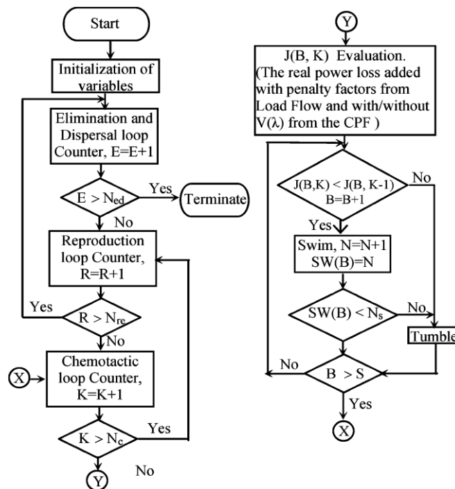
Fig.1. Flowchart of the bacteria foraging algorithm.
