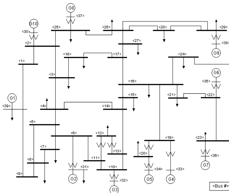
Fig4. New England power system layout
