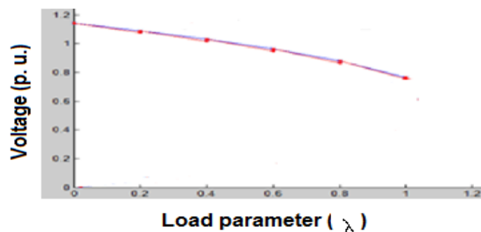
Fig6: PV curve of weakest bus (simultaneous UPFC and tap)
