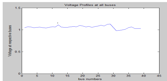
Fig5: Voltage profiles of all the buses at nominal load
