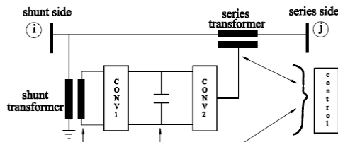
Fig2: The UPFC device circuit arrangement
