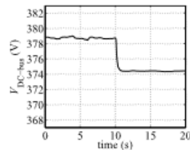
Fig. 20. Case B: dc bus voltage profile.
