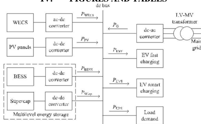
Fig. 1. Layout of the dc microgrid
