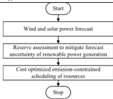
Fig. 3. Overview of optimized scheduling approach.
