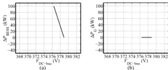
Fig. 16. Case A: BESS and grid droop response curves. (a) Droop response curve of BESS. (b) Droop response curve of grid.
