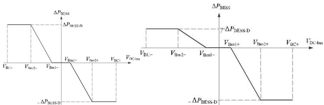
Fig. 7. Droop control of BESS power electronic converter to mitigate deviations of dc microgrid in normal SOC of the BESS.
